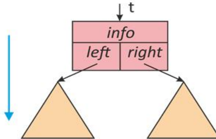
Pre-order
