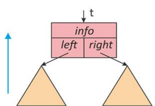
Post-order
